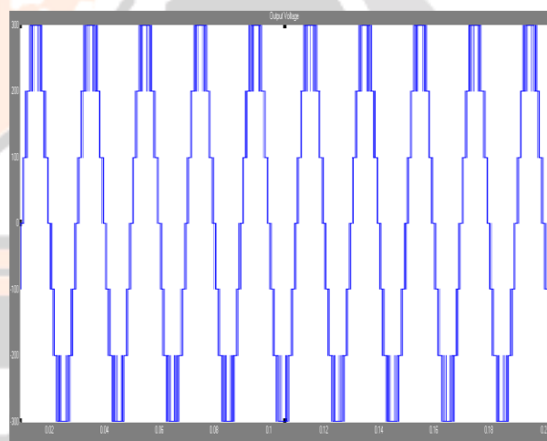
Fig. 12: Output voltage for a 7-level IPD- MLI
