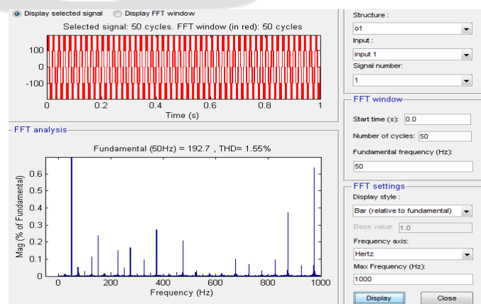
Fig. 13: THD on a Output voltage for a 5-level IPD- MLI
