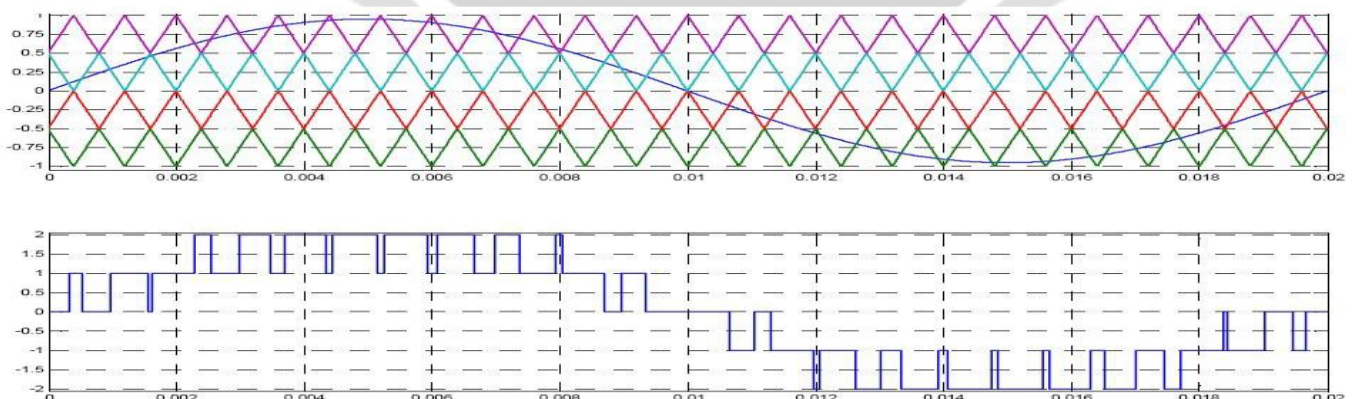
Fig. 7: Level Shifted PWM carriers and reference for a 5-level converter, Alternative Phase Opposition Disposition (APOD).
