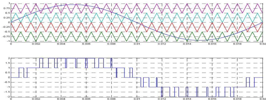
Fig.6: LSPWM carriers and reference for a 5-level converter, Phase Opposition Disposition (POD)
