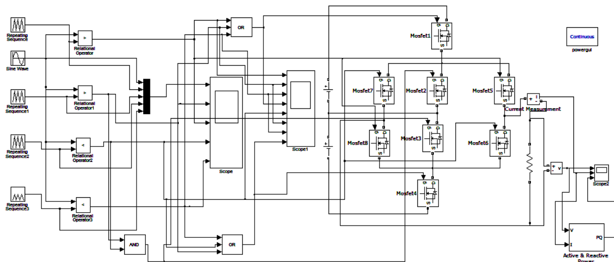
Fig.10 5-Level SPWM Inverter Simulation Circuit.
