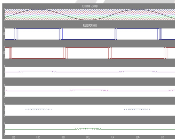
Fig. 15: Gate Pulse for a 7-level IPD- MLI
