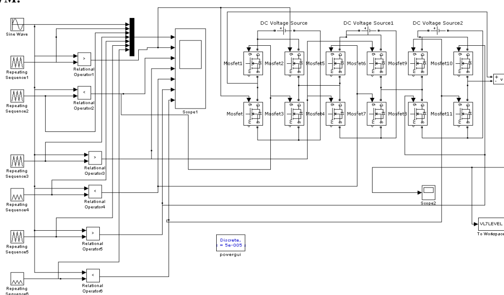
Fig.14. 7-Level SPWM Inverter Simulation Circuit.
