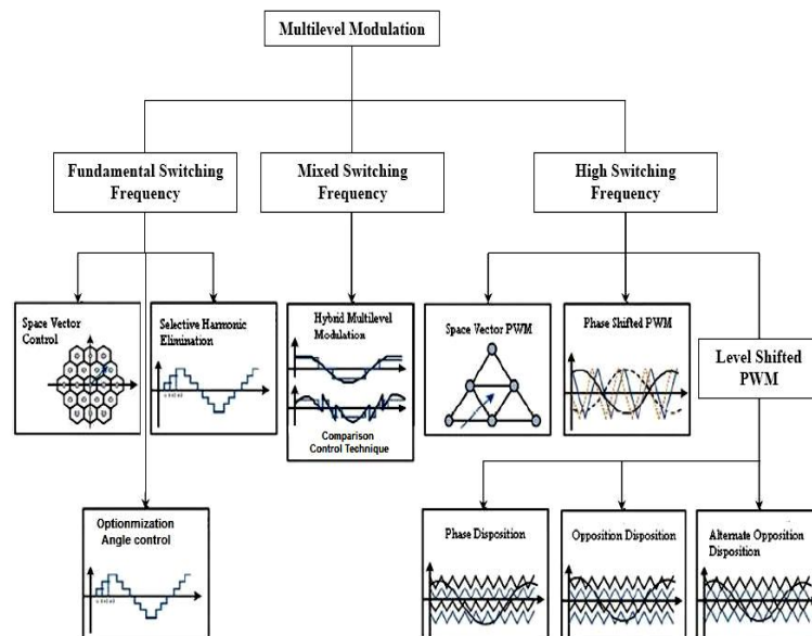
Fig.4: Classification tree for multilevel modulations.
