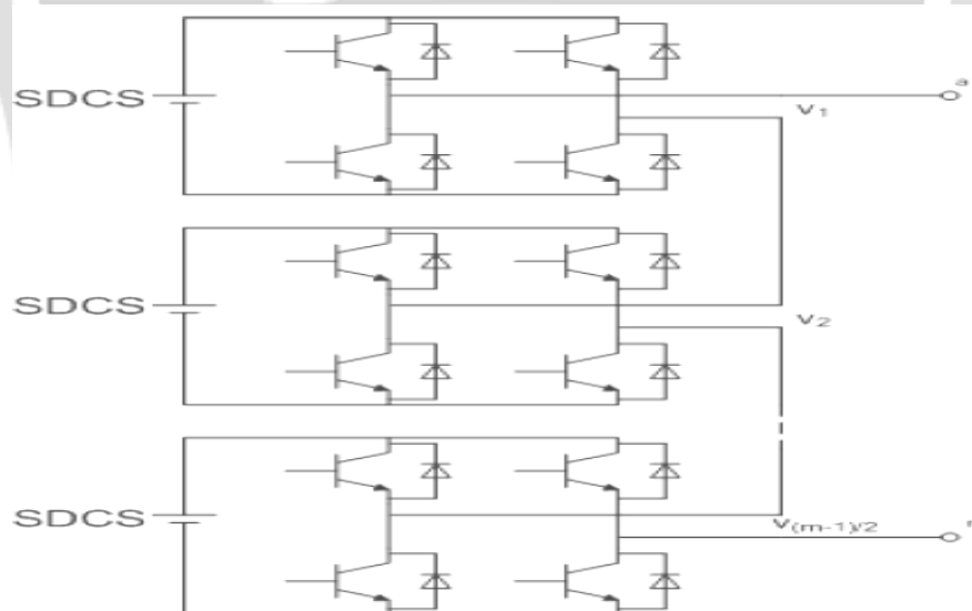
Fig. 3: CHB multilevel inverter topology.
