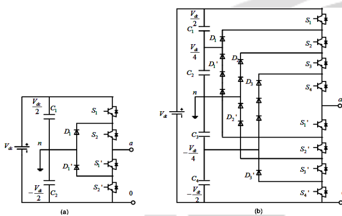
Fig. 1: Diode-clamped multilevel inverter topologies: (a) Three-level. (b) Five-level.
