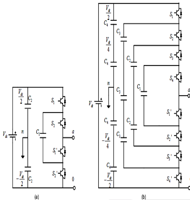
Fig. 2: Diode-clamped multilevel inverter topologies: (a) Three-level.(b) Five-level.
