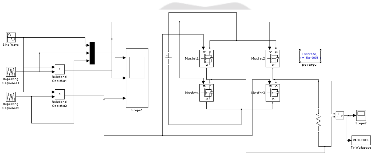
Fig.8 3-Level SPWM Inverter Simulation Circuit.
