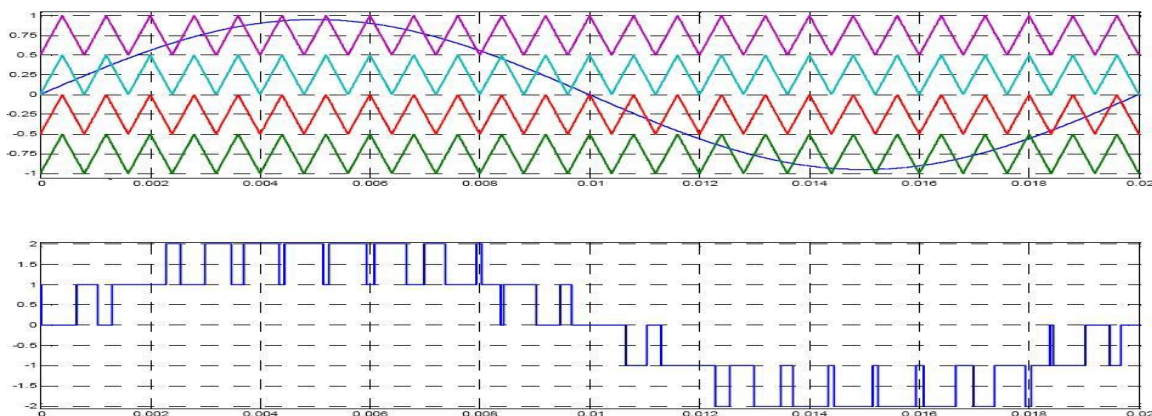
Fig. 5: LSPWM carriers and reference for a 5-level converter, In Phase Disposition (IPD)
