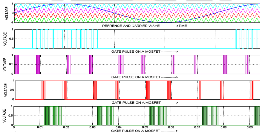
Fig. 11: LSPWM carriers and reference for a 5-level converter, and variance gate pulse on Mosfet In Phase Disposition (IPD) MLI
