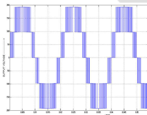
Fig. 12: Output voltage for a 5-level IPD- MLI
